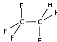
HFC-134a
