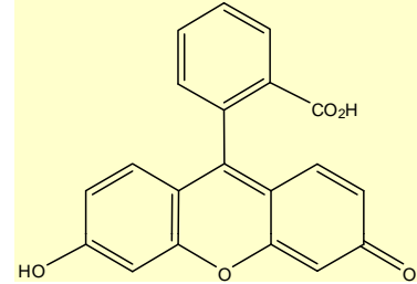
Fluoresceina
