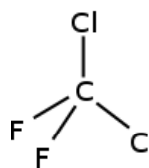
CFC-12
